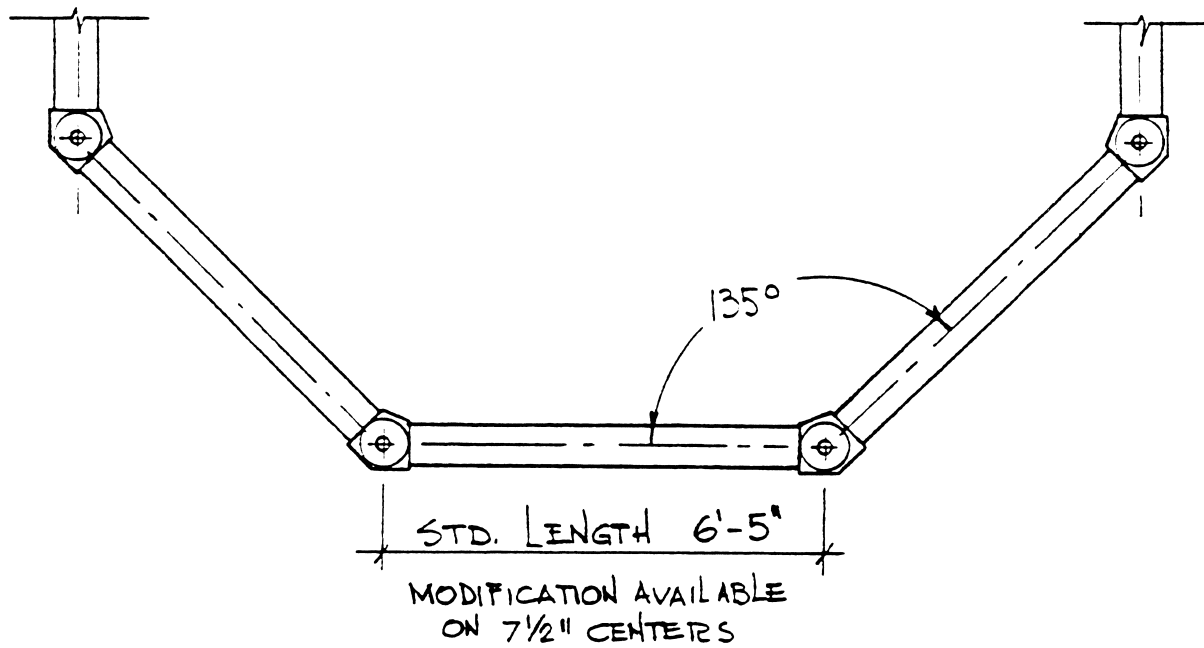
PLAN VIEW OF BALUSTRADE
