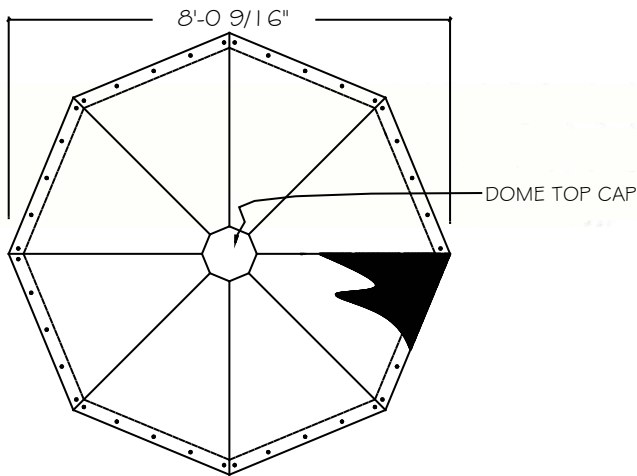
DOME PLAN DETAIL
