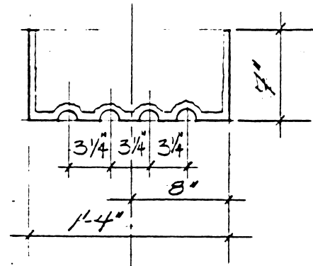
A SECTION THRU COLUMN SHAFT
