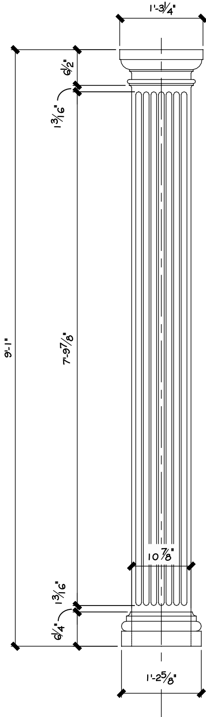
ELEV. OF EP-137 PILASTER
