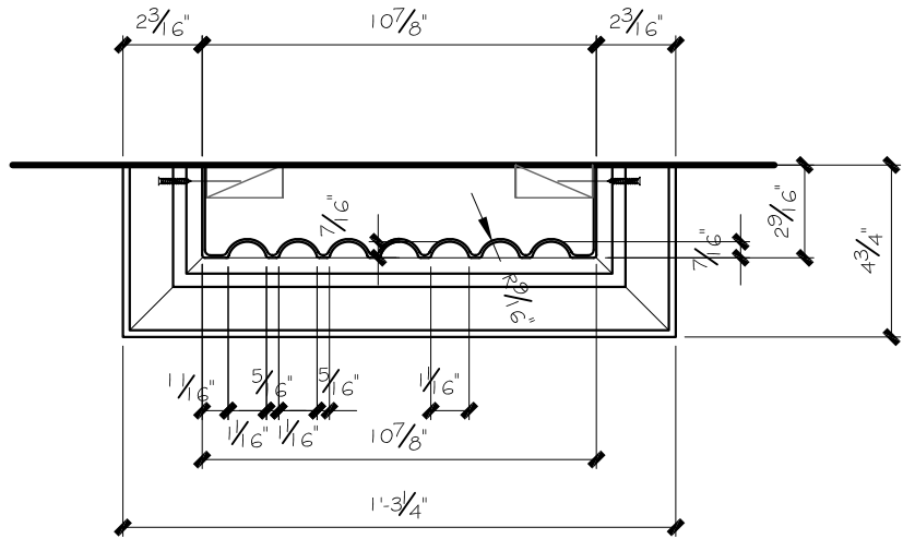
REFLECTED PLAN OF CAPITAL
